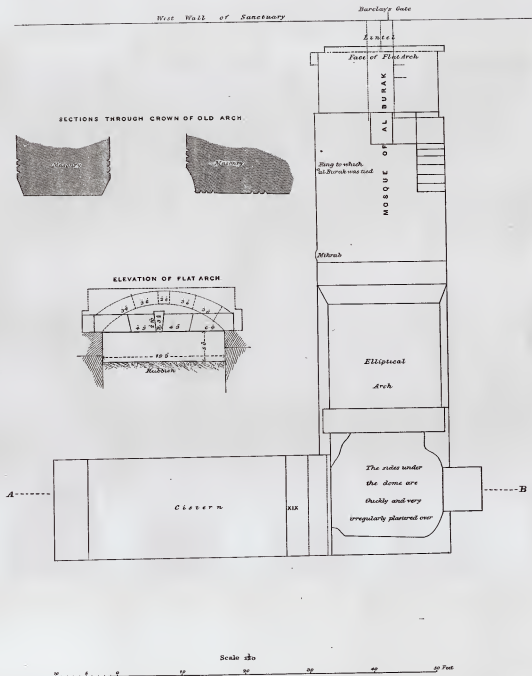
Scale 1/2"
